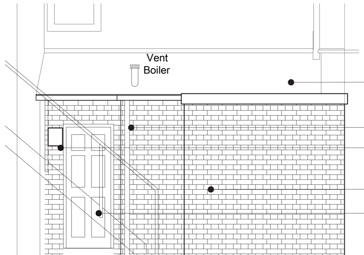
PROPOSED ELEVATIONS WITH REMODELLED EXTENSION (RES736-BHA-00-ZZ-DR-A-3003)
